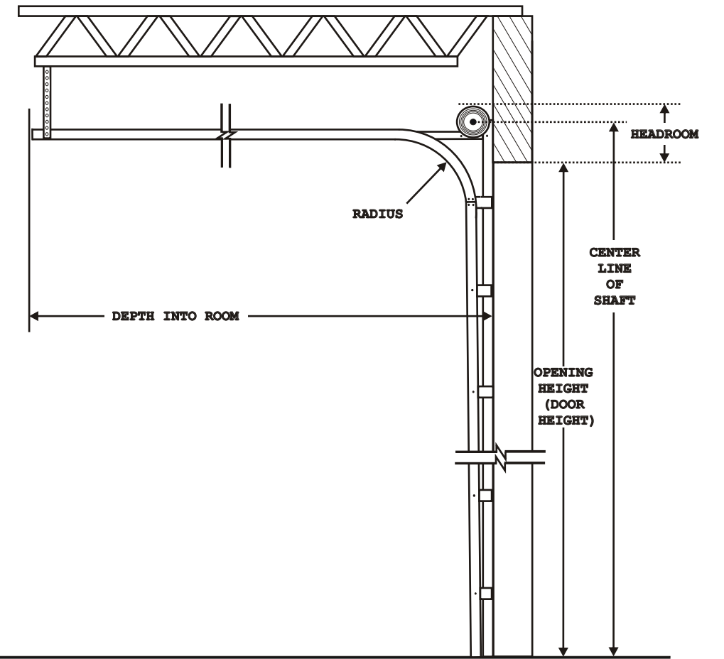
SIDE VIEW OF TRACK
