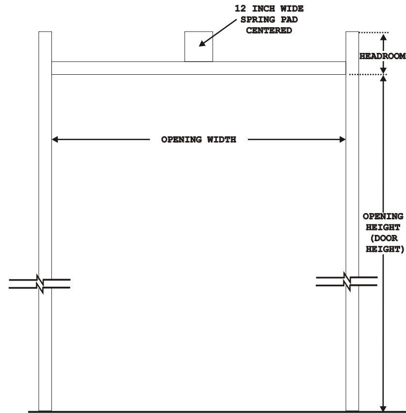
INTERIOR ELEVATION
